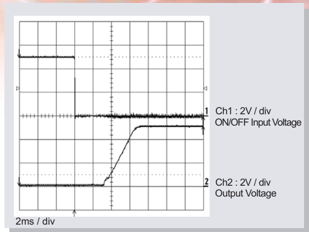
Fig13. Start-up Using Remote ON/OFF with Prebias ( V_o = 5V , I_o = 10A )
