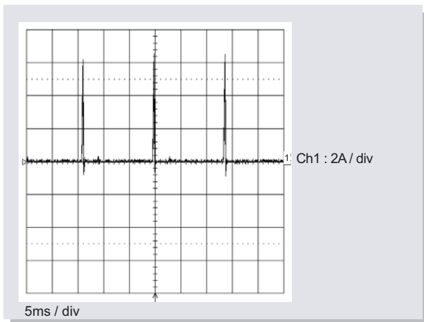
Fig16. Input Current with Short Circuit at Output ( V_o = 5V , I_o = 10A )
