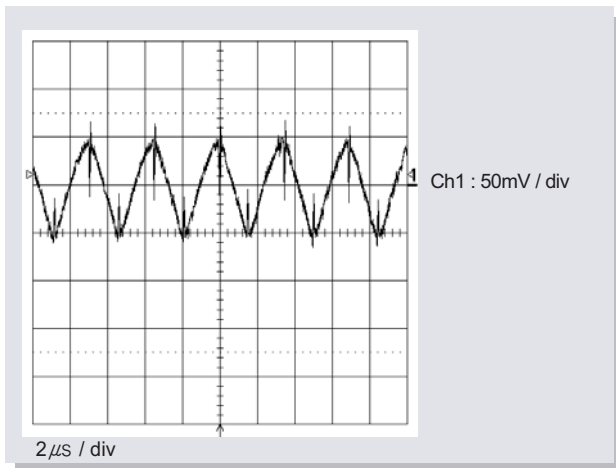
Fig14. Input Reflected Ripple Voltage ( V_o = 5V , I_o = 10A , C_{in} = 100\mu F \times 2 , L_{in} = 1\mu F )
