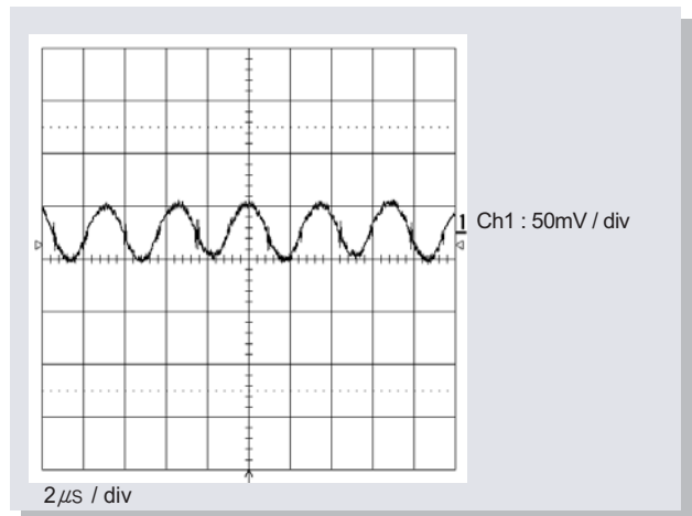
Fig15. Output Voltage Ripple & Noise ( V_o = 5V , I_o = 10A )
