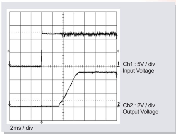
Fig12. Start-up with Application of Vin ( V_o = 5V , I_o = 10A )
