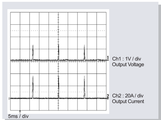
Fig17. Output Current & Voltage with short Circuit at Output ( V_o = 5V , I_o = 10A )
