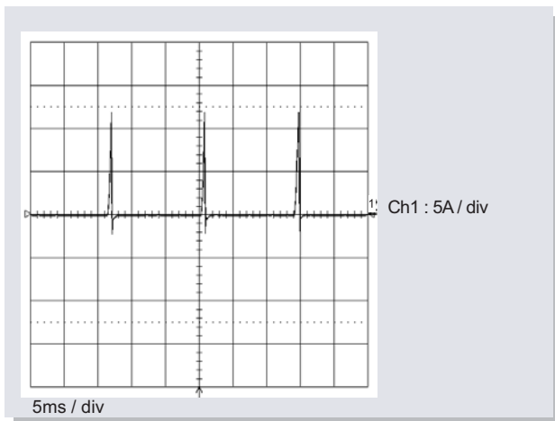
Fig16. Input Current with Short Circuit at Output ( V_o = 5V , I_o = 15A )
