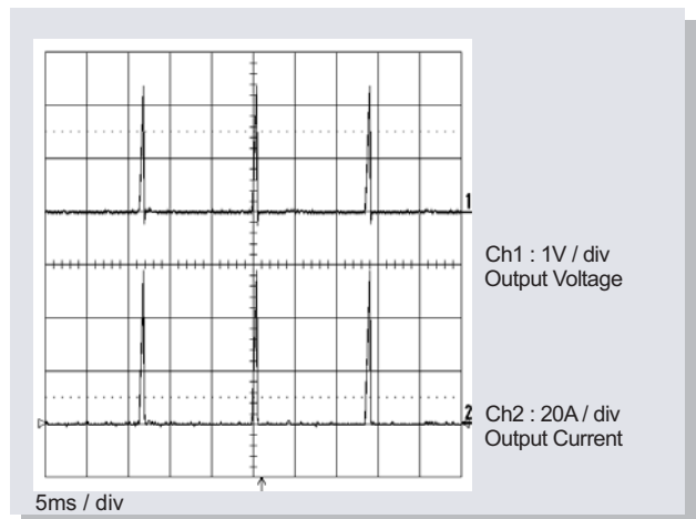
Fig17. Output Current & Voltage with short Circuit at Output ( V_o = 5V , I_o = 15A )
