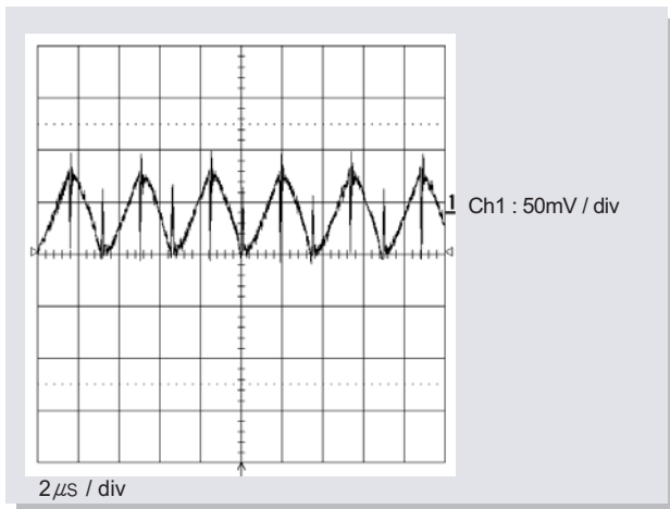
Fig14. Input Reflected Ripple Voltage ( V_o = 5V , I_o = 15A , C_{in} = 100\mu F \times 2 , L_{in} = 1\mu F )
