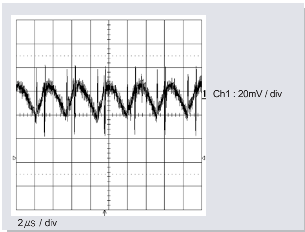
Fig14. Input Reflected Ripple Voltage ( V_o = 3.3V , I_o = 15A , C_{in} = 100\mu F \times 2 , L_{in} = 1\mu F )
