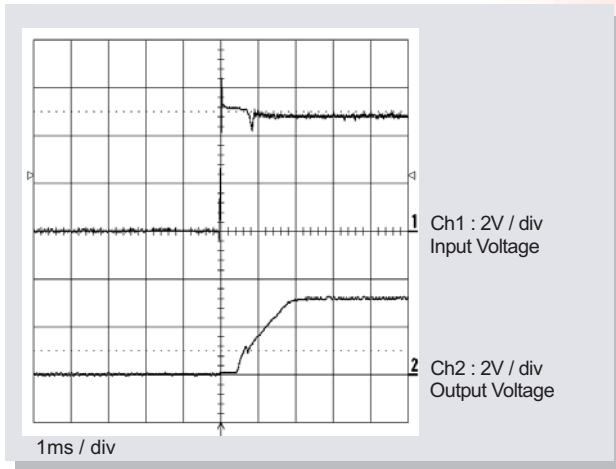
Fig12. Start-up with Application of Vin ( V_o = 3.3V , I_o = 15A )
