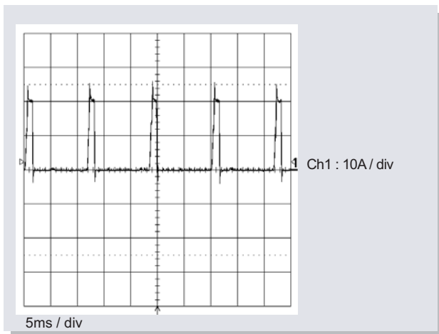
Fig16. Input Current with Short Circuit at Output ( V_o = 3.3V , I_o = 15A )
