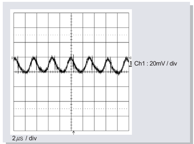
Fig15. Output Voltage Ripple & Noise ( V_o = 3.3V , I_o = 15A )
