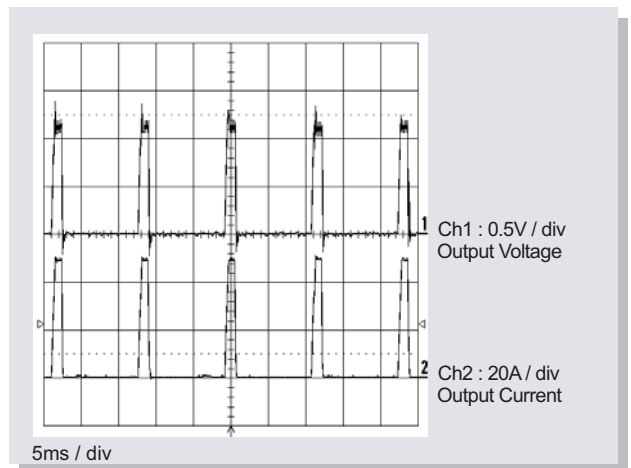
Fig17. Output Current & Voltage with short Circuit at Output ( V_o = 3.3V , I_o = 15A )
